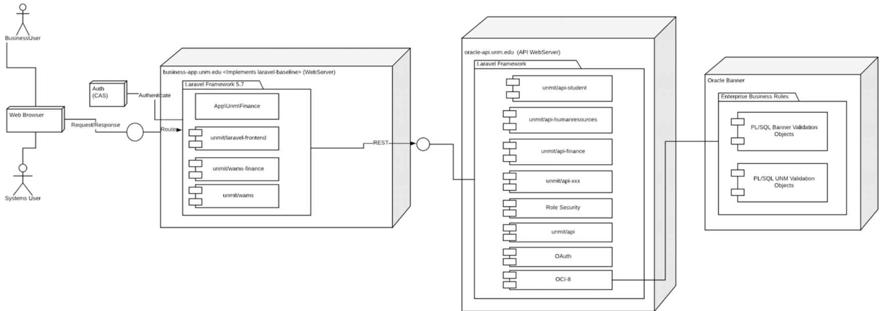
RESTful-Deployment Diagram
